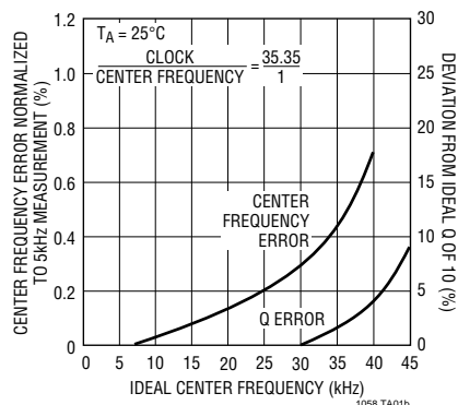
Center Frequency and Q Error
