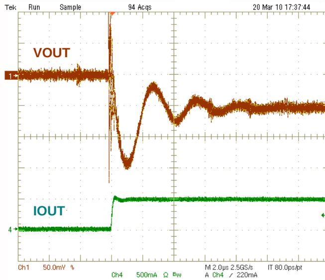
LOAD TRANSIENT
