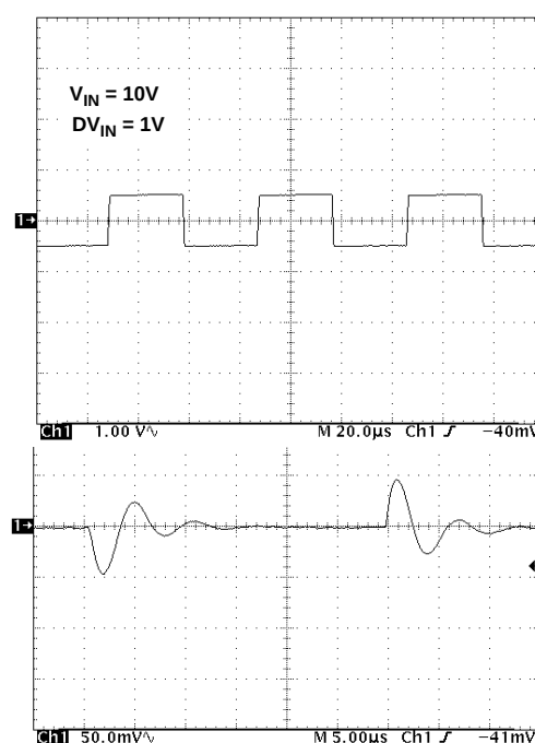
FIGURE 52. LINE TRANSIENT RESPONSE, 0.001µF LOAD CAPACITANCE
