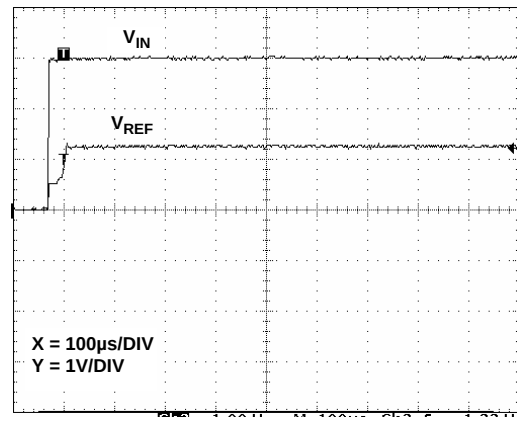
FIGURE 11. TURN-ON TIME
