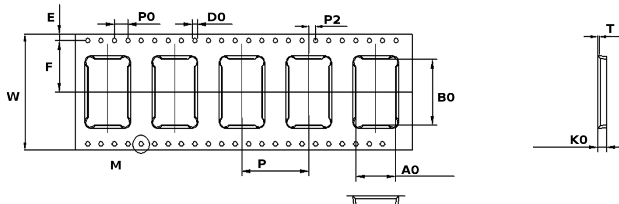
Figure 15 - Tape Specifications
