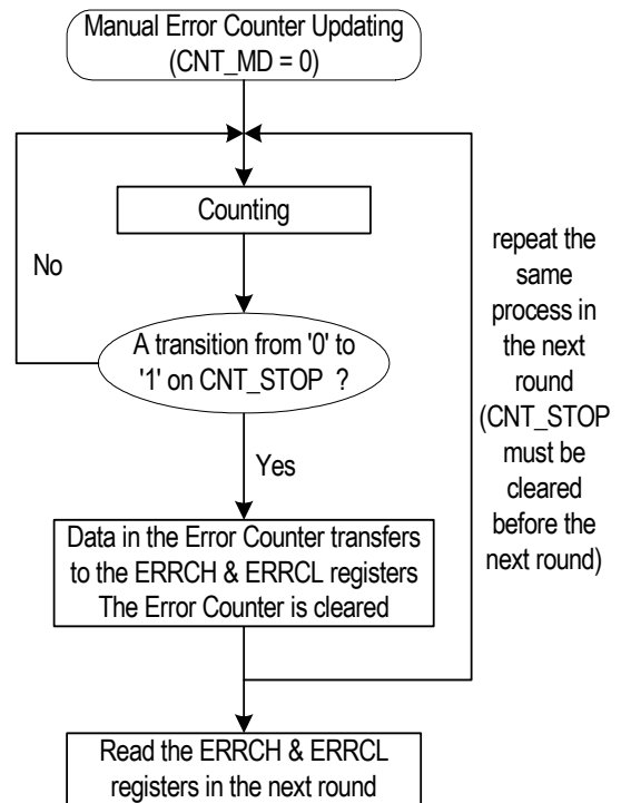
Figure-22 Manual Error Counter Updating
