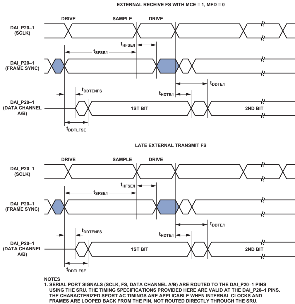
Figure 20. External Late Frame Sync 1
