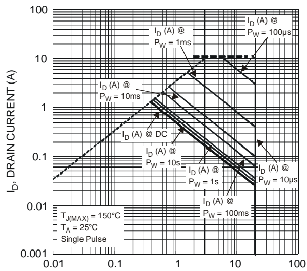
Fig. 2 SOA, Safe Operation Area
