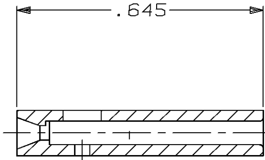
SECT X-X
