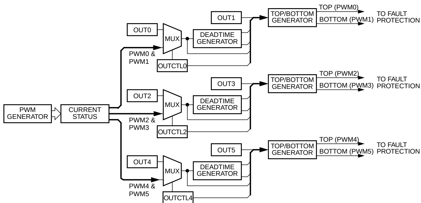
Figure 14-50. Deadtime Generators
