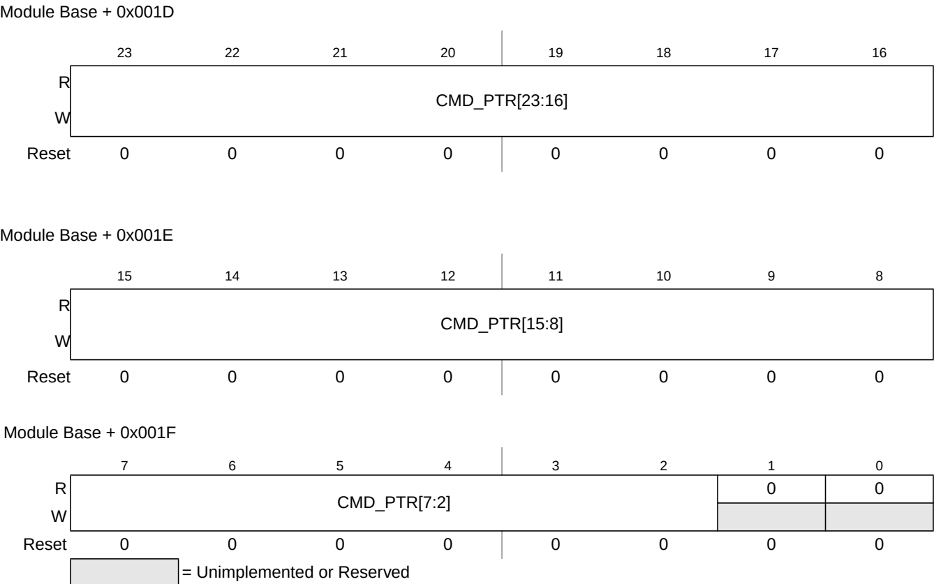
Figure 9-23. ADC Command Base Pointer Registers (ADCCBP_0, ADCCBP_1, ADCCBP_2))
