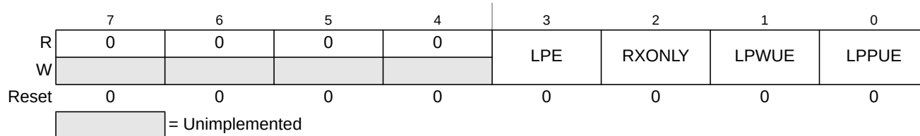
Figure 18-4. LIN Control Register (LPCR)
