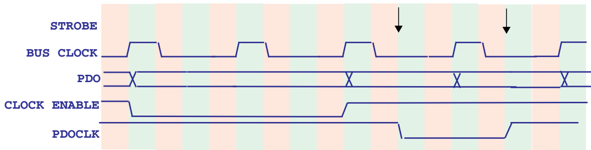
Figure 6-31. PDO Profiling Clock Control
