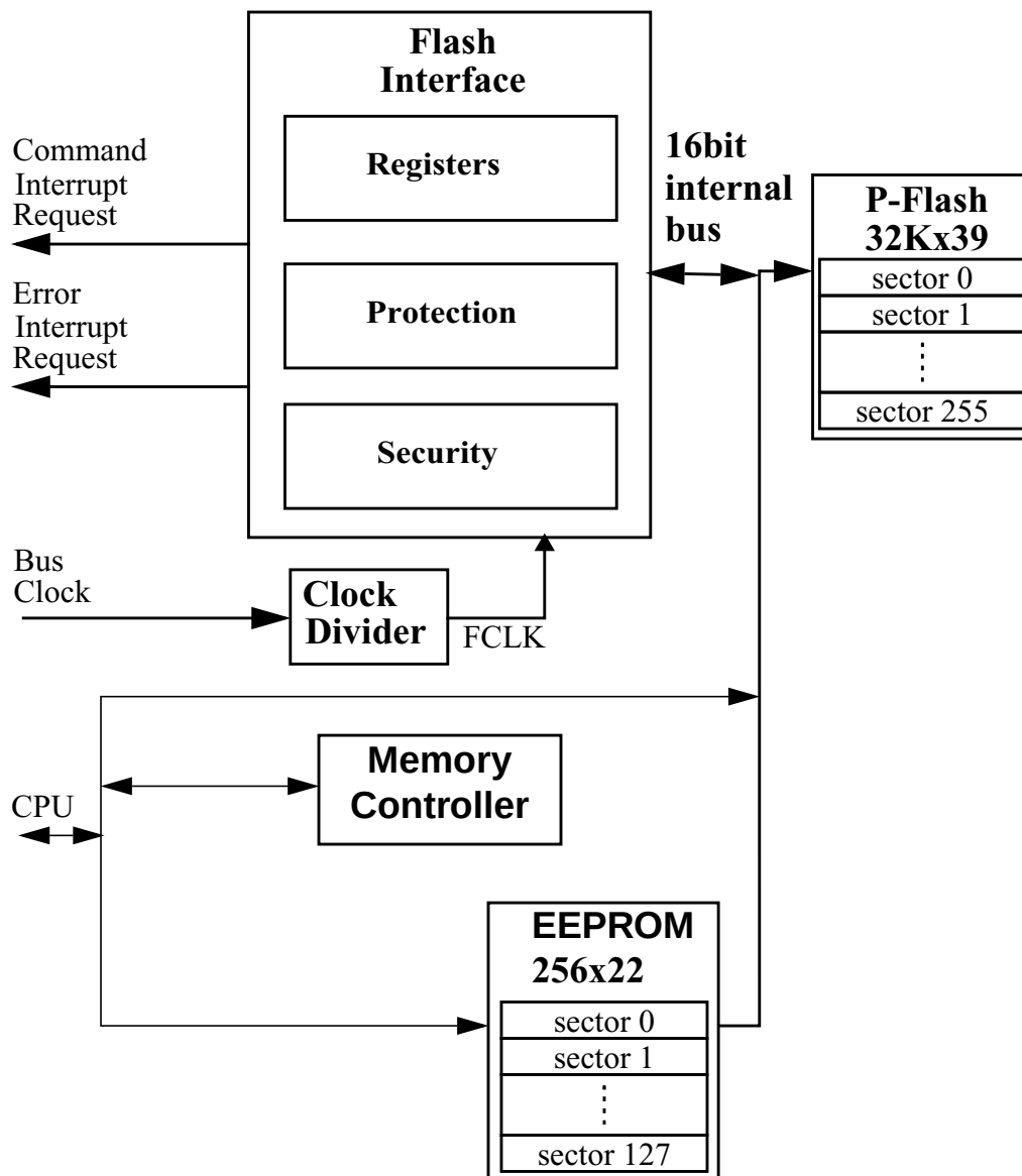
Figure 19-1. FTMZR128K512 Block Diagram
