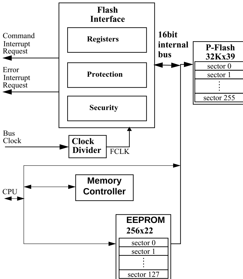
Figure 19-1. FTMZR128K512 Block Diagram
