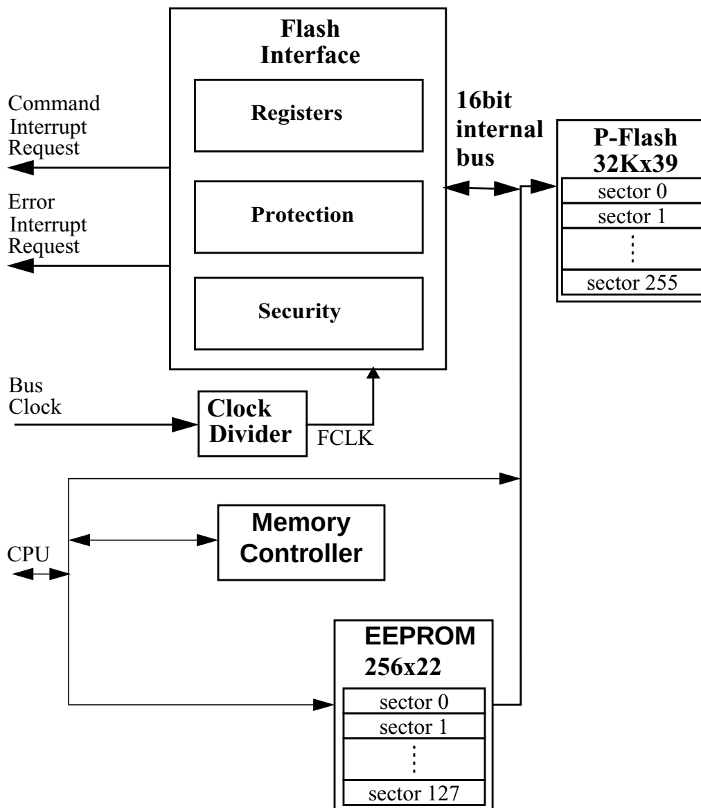
Figure 19-1. FTMZR128K512 Block Diagram
