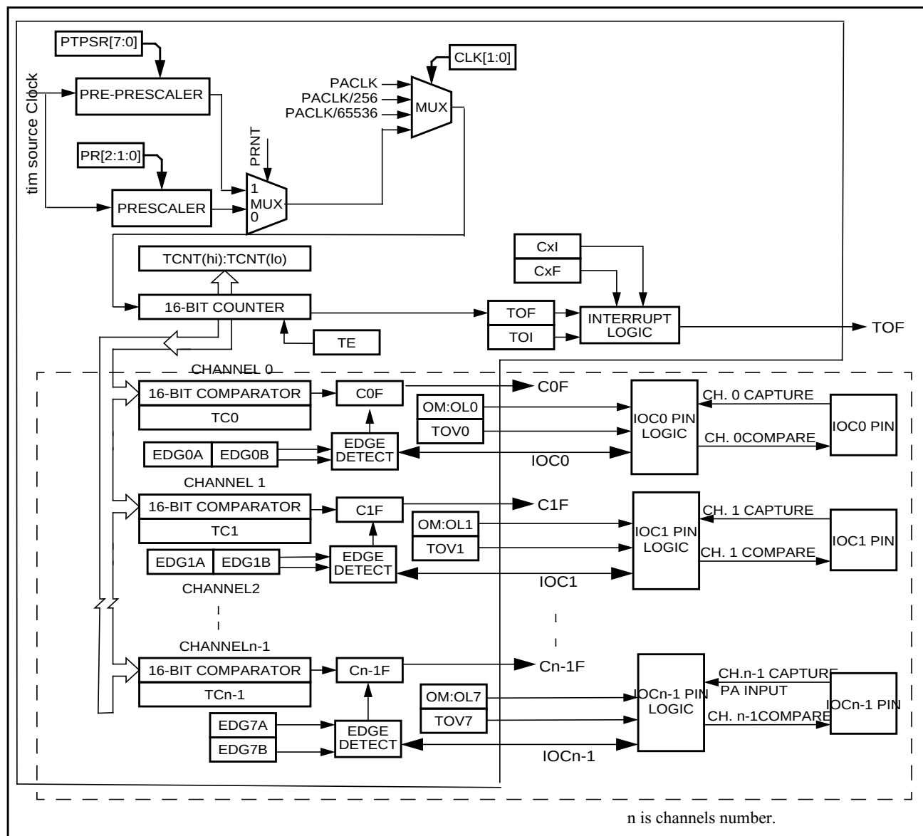
Figure 11-22. Detailed Timer Block Diagram
