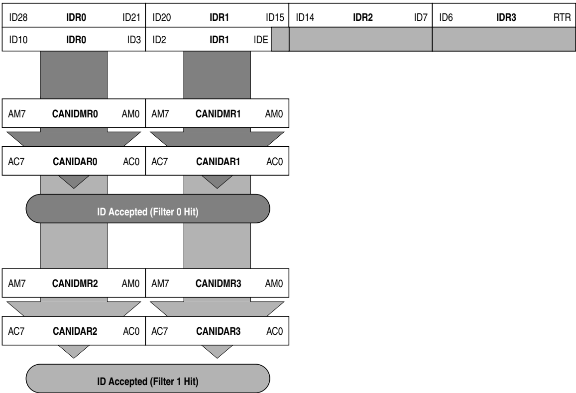
Figure 12-41. 16-bit Maskable Identifier Acceptance Filters
