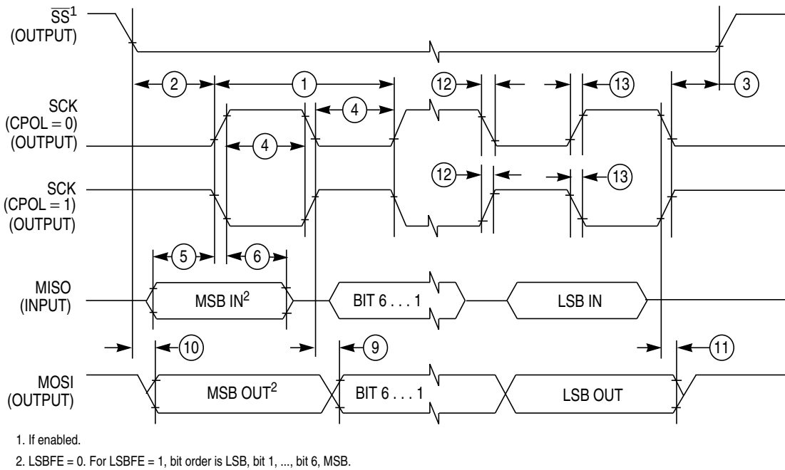
Figure H-2. SPI Master Timing (CPHA=0)
