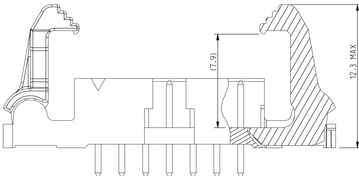
SECTION C-C
