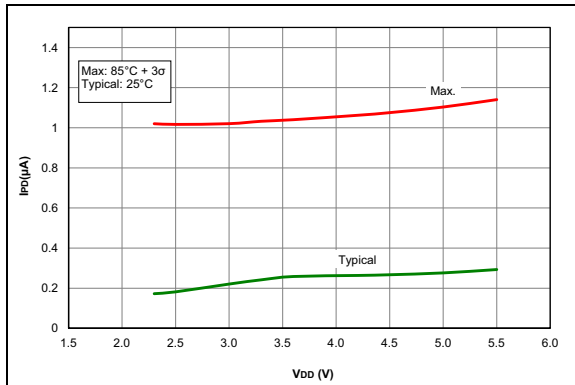
FIGURE 36-38: I_{PO} , ADC Non-Converting, PIC16F1615/9 Only.
