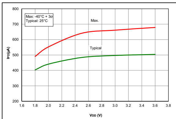
FIGURE 36-39: I_{PO} , Comparator, NP Mode ( CxSP = 1 ), PIC16LF1615/9 Only.
