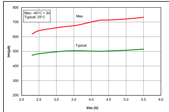
FIGURE 36-40: I_{PO} , Comparator, NP Mode ( CxSP = 1 ), PIC16F1615/9 Only.
