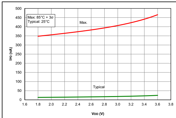
FIGURE 36-37: I_{PO} , ADC Non-Converting, PIC16LF1615/9 Only.
