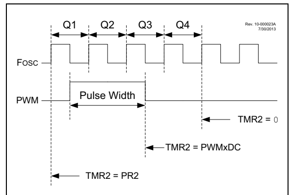
FIGURE 27-2: PWM OUTPUT
