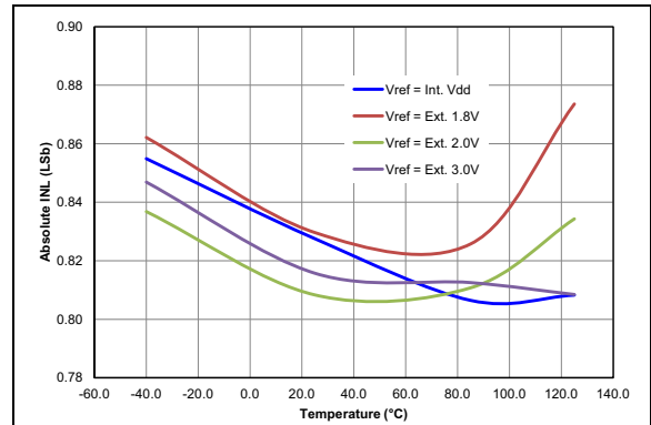
FIGURE 36-102: Absolute Value of DAC INL Error, V_{DD} = 3.0V , V_{REF} = V_{DD} .
