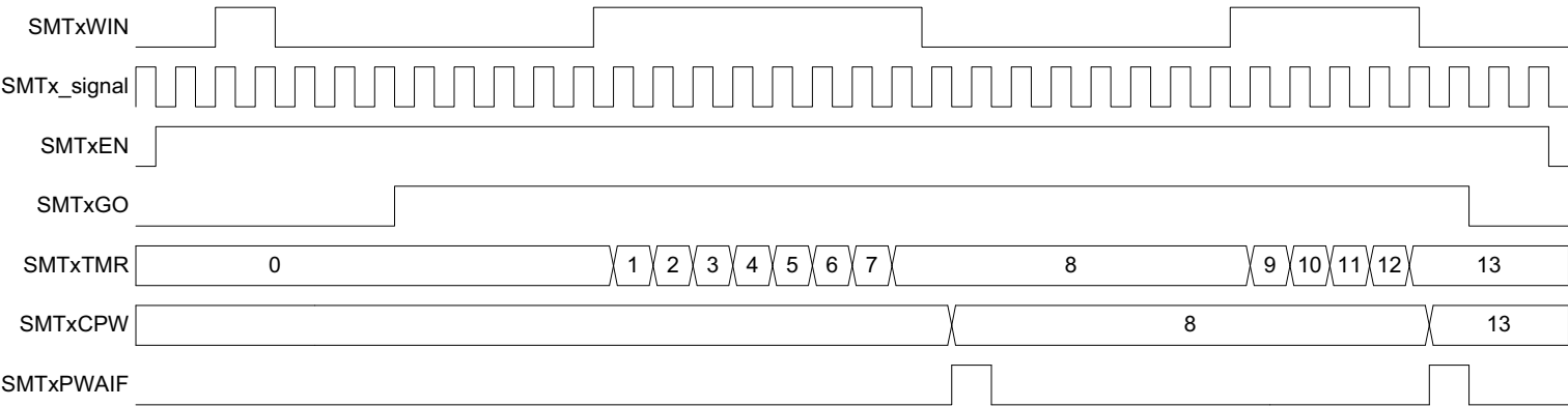
FIGURE 29-20: GATED COUNTER MODE SINGLE ACQUISITION TIMING DIAGRAM
