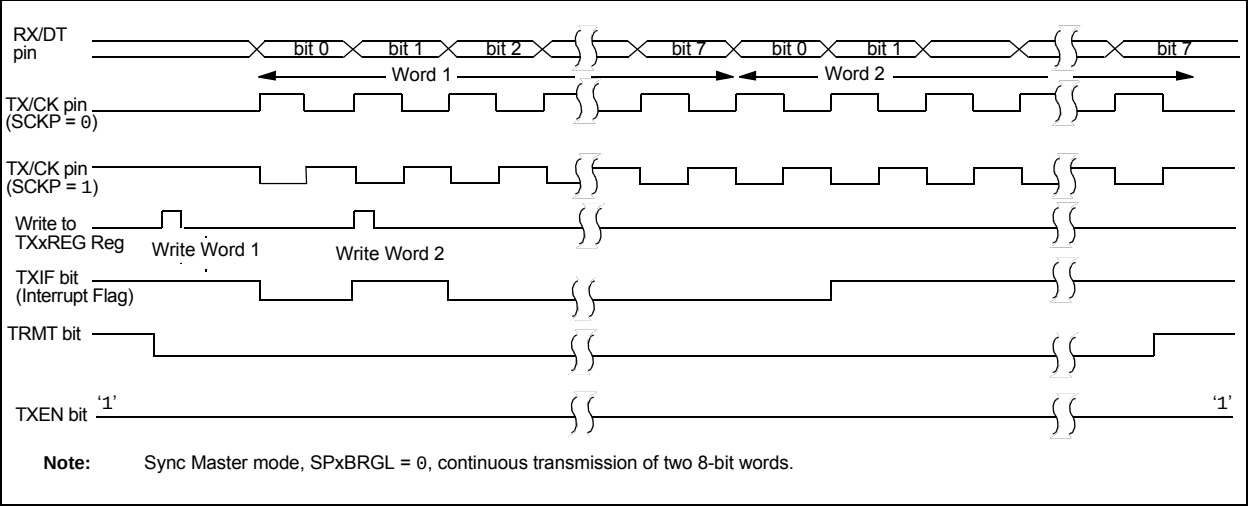
FIGURE 25-11: SYNCHRONOUS TRANSMISSION (THROUGH TXEN)
