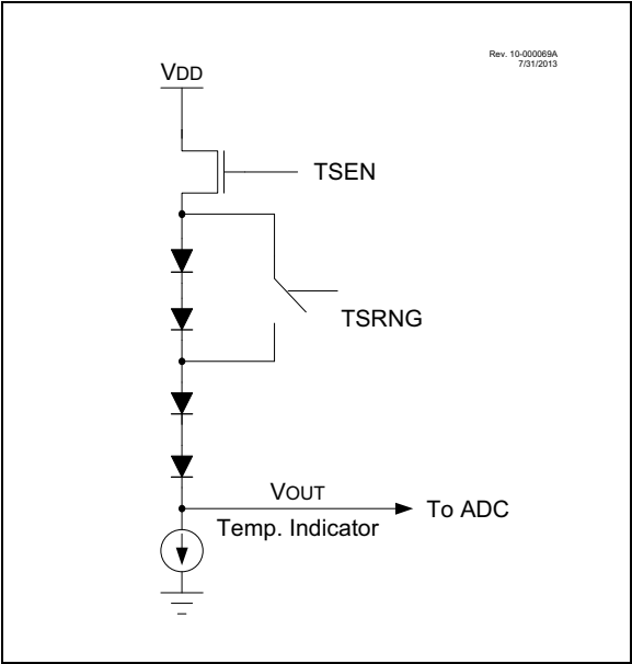
FIGURE 16-1: TEMPERATURE CIRCUIT DIAGRAM
