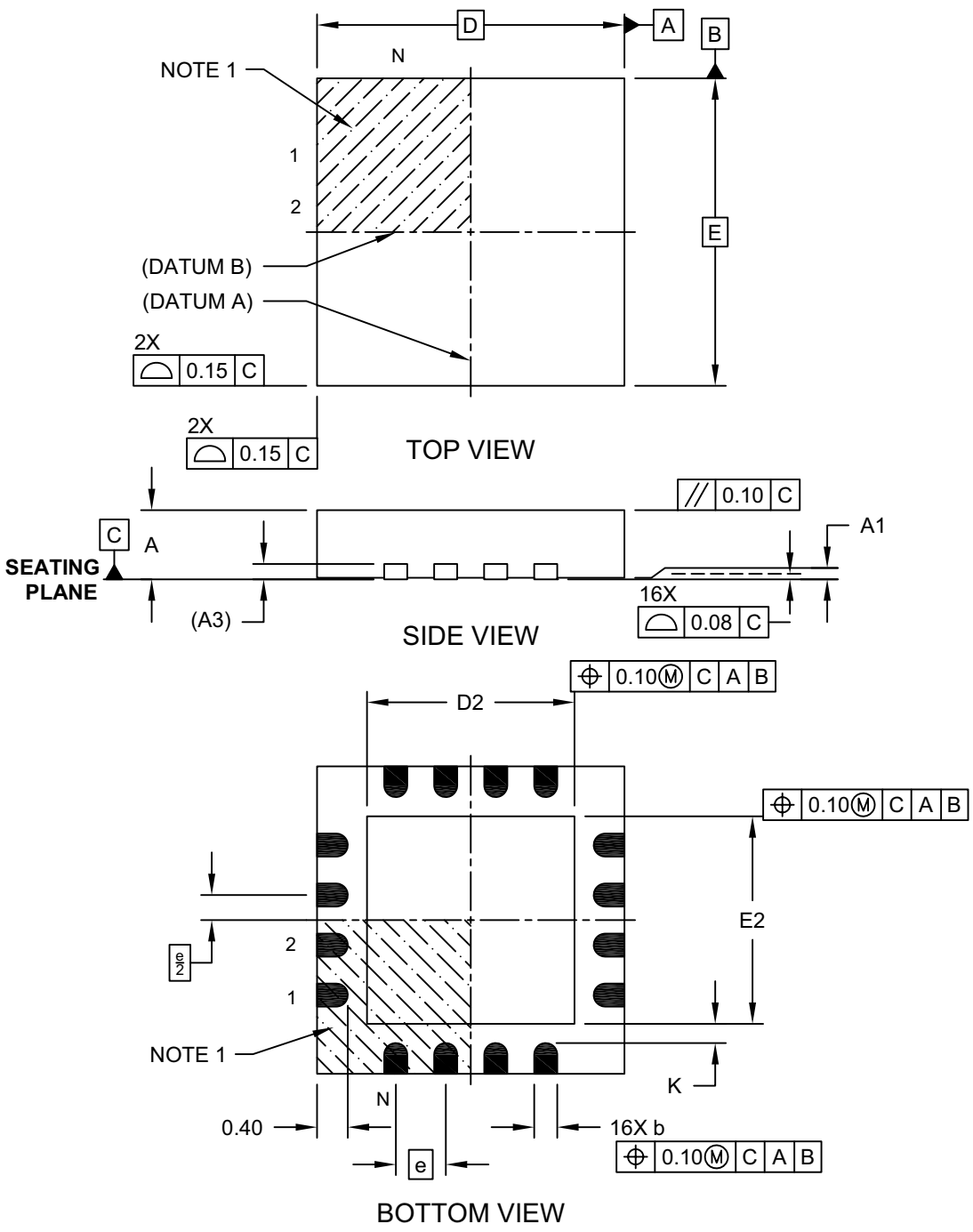
Microchip Technology Drawing C04-127D Sheet 1 of 2
