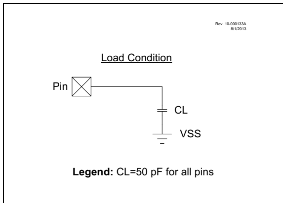
FIGURE 35-4: LOAD CONDITIONS
