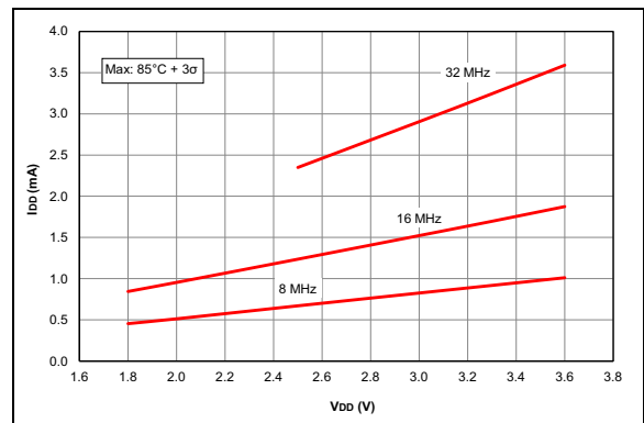
FIGURE 36-18: I_{DD} Maximum, HFINTOSC Mode, PIC16LF1615/9 Only.
