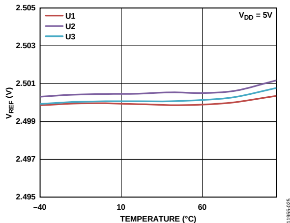
Figure 25. Internal Reference Voltage vs. Temperature (Grade B)
