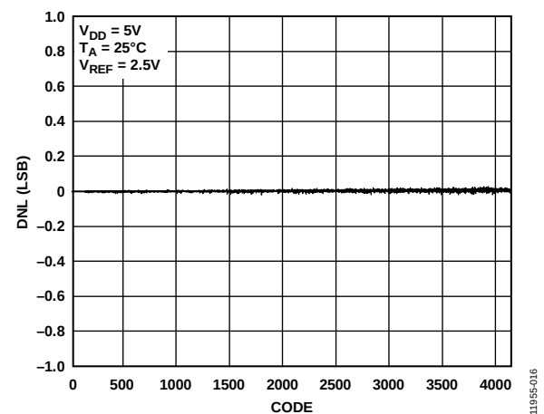
Figure 16. AD5681R DNL
