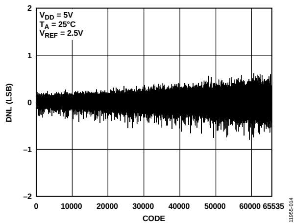
Figure 14. AD5683R/AD5683 DNL
