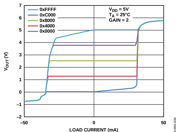
Figure 39. Source and Sink Capability, Gain = 2
