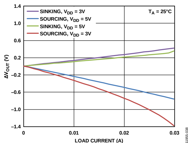
Figure 38. Headroom/Footroom vs. Load Current
