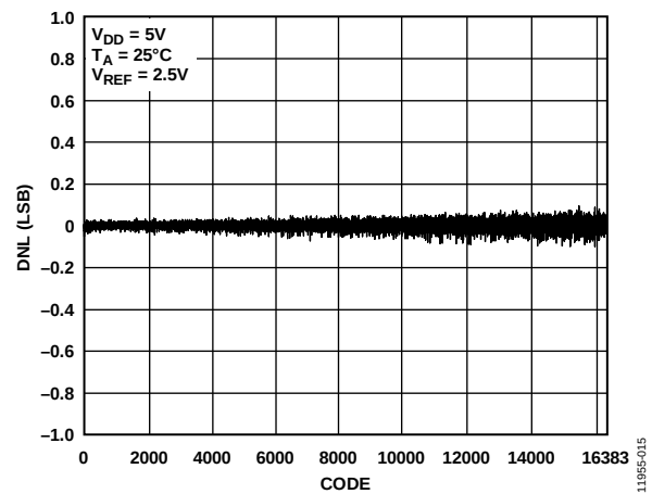
Figure 15. AD5682R DNL
