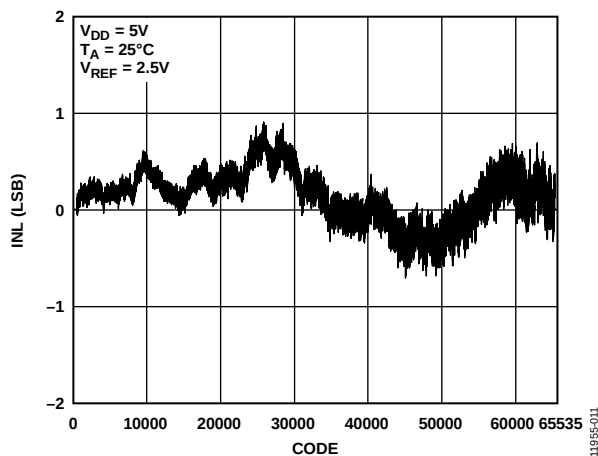
Figure 11. AD5683R/AD5683 INL
