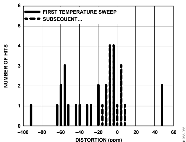
Figure 54. Thermal Hysteresis
