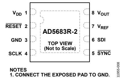
Figure 8. Pin Configuration, 8-Lead LFCSP, RESET Option
