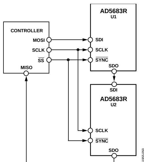
Figure 50. Daisy-Chain Connection
