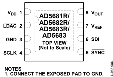
Figure 6. Pin Configuration, 8-Lead LFCSP, \overline{LDAC} Option
