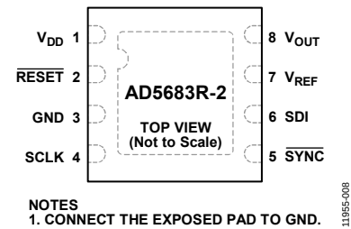
Figure 8. Pin Configuration, 8-Lead LFCSP, \overline{RESET} Option
