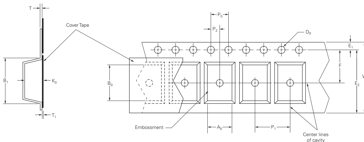
Figure S18 — EIA Referenced Taped Component Dimensions
