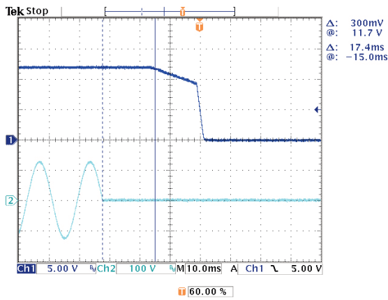
Figure 5 ECP180PS12 90VAC 120W load
