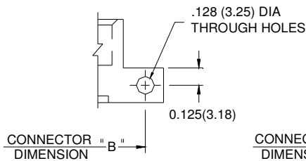
MOUNTING OPTION CODE x12 (SIDE MOUNTING HOLES)
