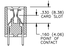
DUAL ROW
