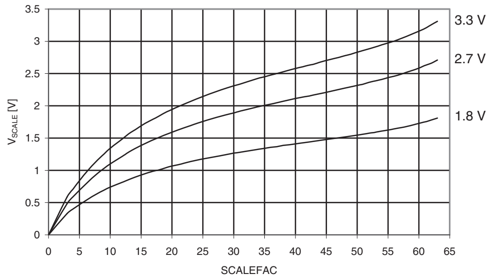
Figure 36-1. Analog Comparator Voltage Scaler vs. Scalefac T = 25^{\circ}\text{C}
