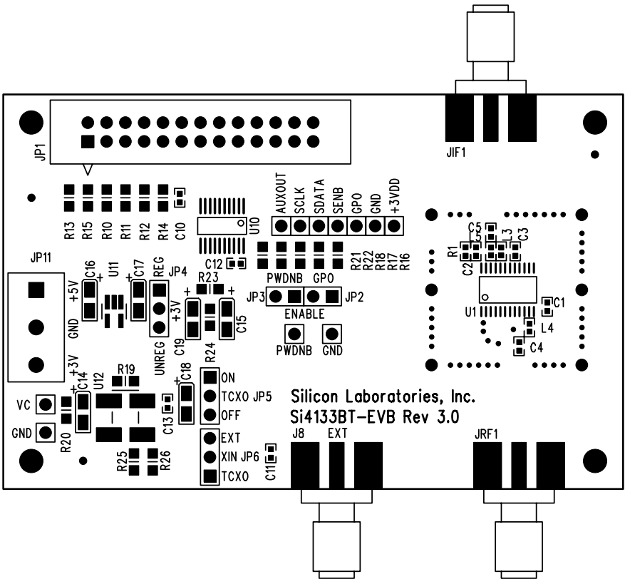
Figure 21. Si4133BT Silkscreen
