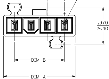
CIRCUIT NO. 1
