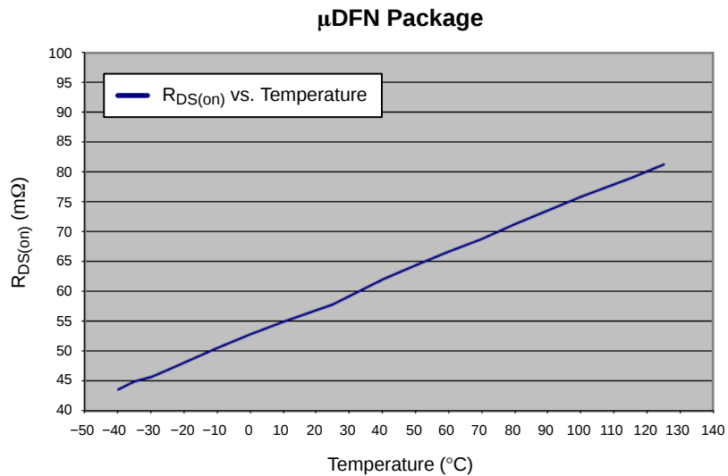
Figure 21. R_{DS(on)} vs Temperature, μDFN Package
