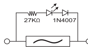
LED Circuit for offline indication in CAFL4UL24V
