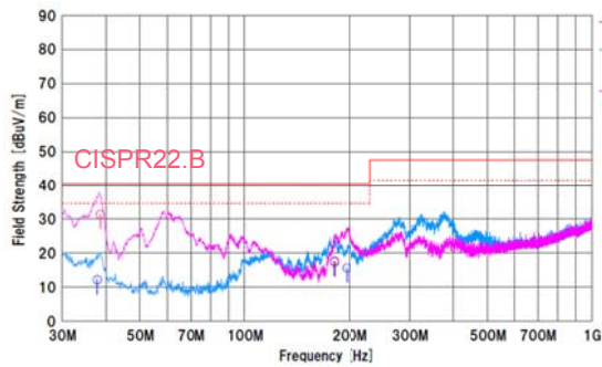
Figure 23. Radiated Emission.1
