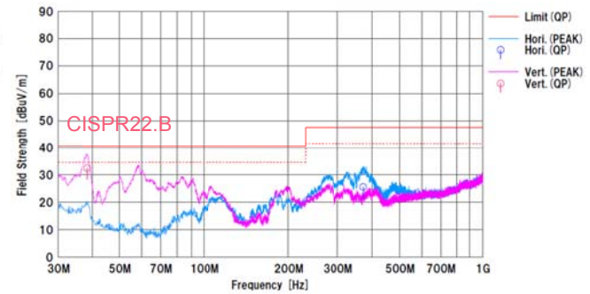
Figure 24. Radiated Emission.2
