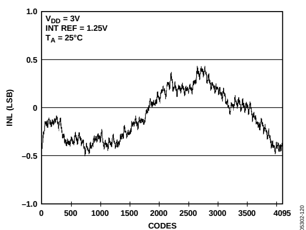
Figure 21. INL AD5628-1
