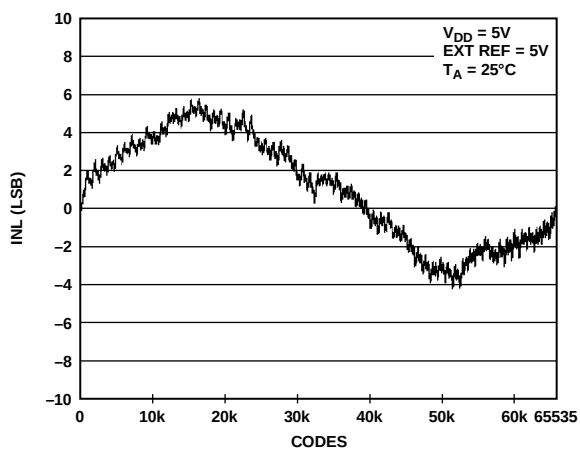
Figure 7. INL AD5668—External Reference
