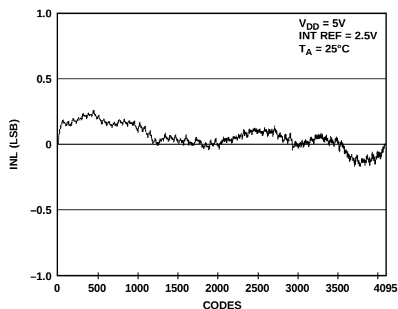
Figure 15. INL AD5628-2
