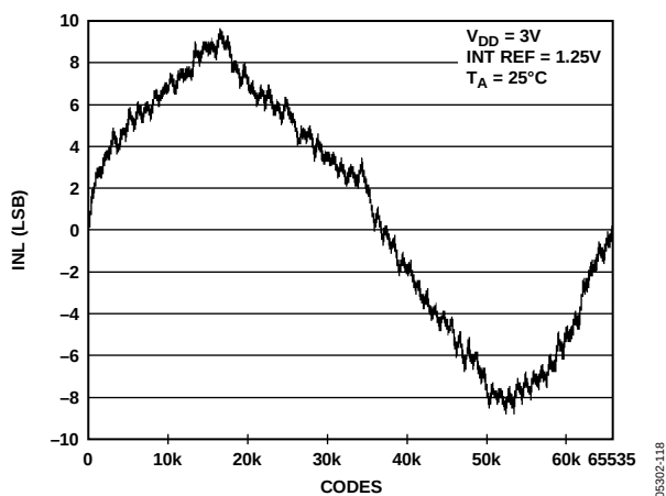
Figure 19. INL AD5668-1
