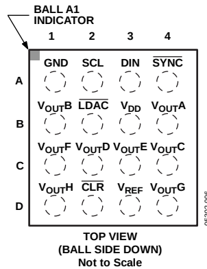
Figure 6. 16-Lead WLCSP
