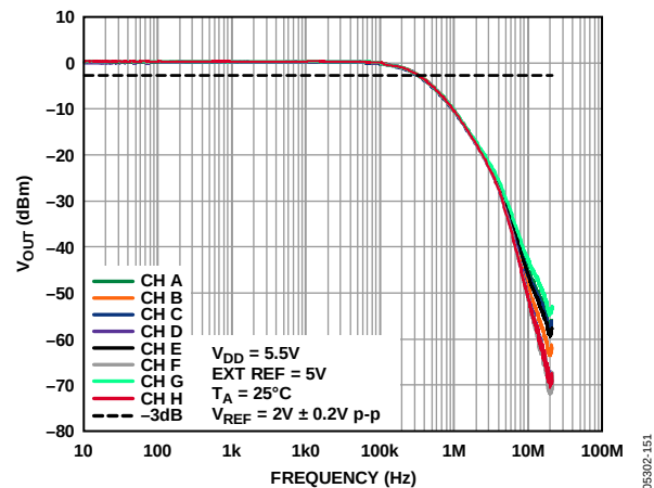
Figure 52. Multiplying Bandwidth
