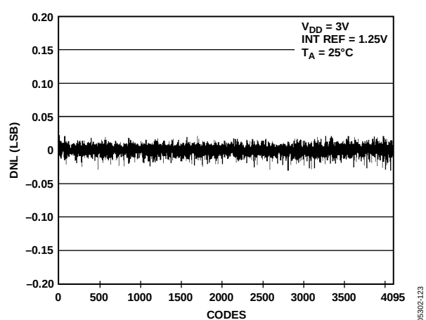
Figure 24. DNL AD5628-1
