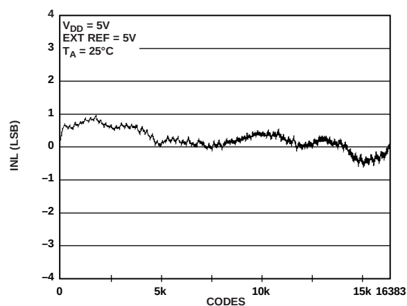
Figure 14. INL AD5648-2
