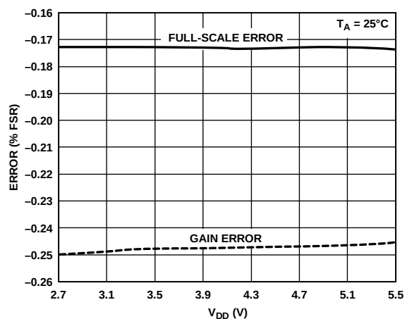
Figure 27. Gain Error and Full-Scale Error vs. Supply Voltage
