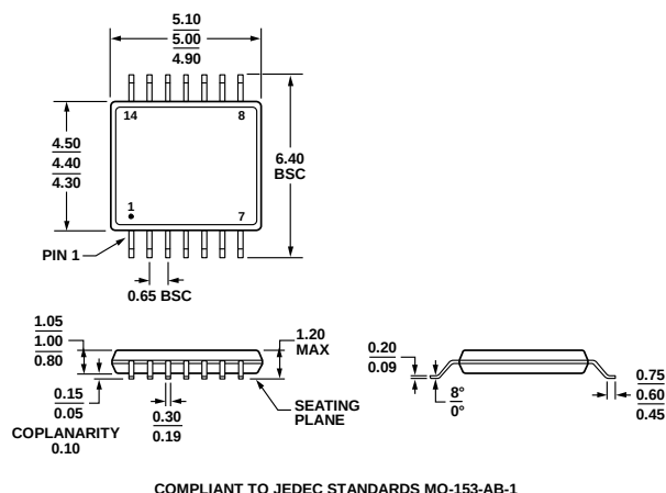
Figure 62. 14-Lead Thin Shrink Small Outline Package [TSSOP] (RU-14)
