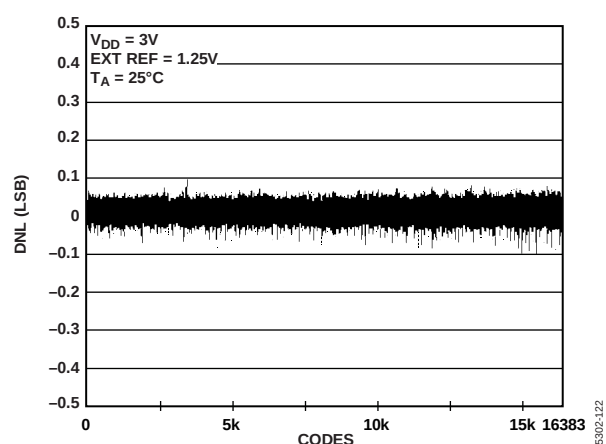
Figure 23. DNL AD5648-1
