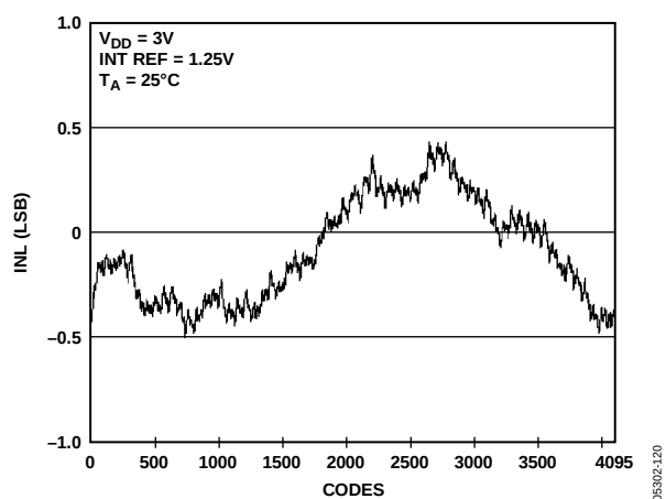
Figure 21. INL AD5628-1
