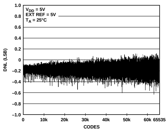
Figure 10. DNL AD5668—External Reference
