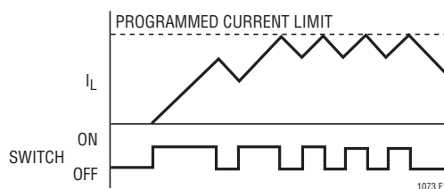
Figure 11. Current Limit Keeps Inductor Current Under Control
