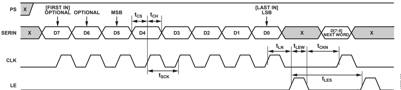
Figure 34. Serial Control Timing Diagram
