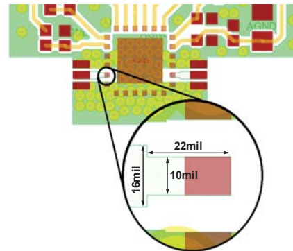
Figure 44. With Impedance Match
