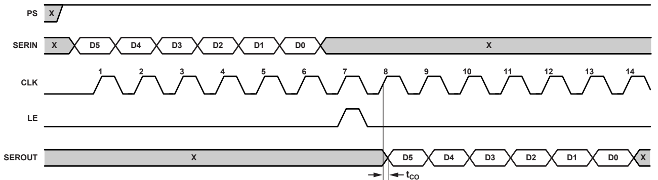
Figure 35. Serial Output Timing Diagram
