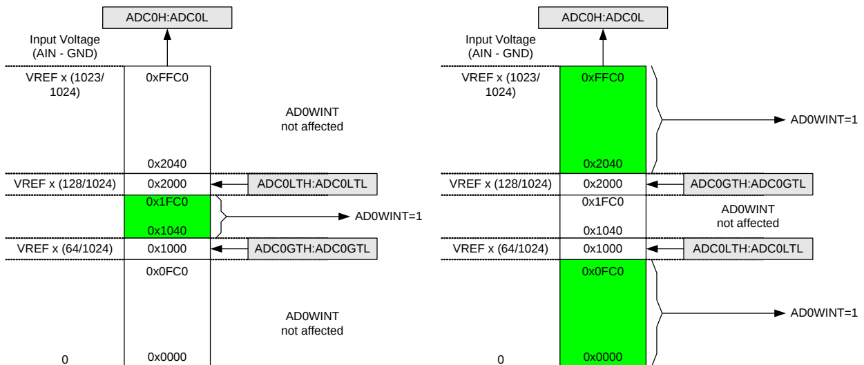
Figure 8.5. ADC Window Compare Example: Left-Justified Data
