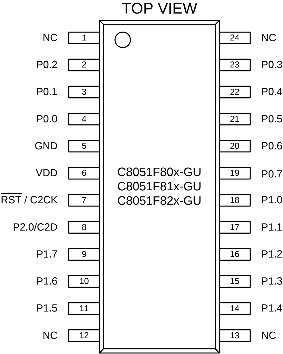
Figure 3.2. QSOOP-24 Pinout Diagram (Top View)
