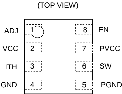
Figure 2. Pin Configuration
