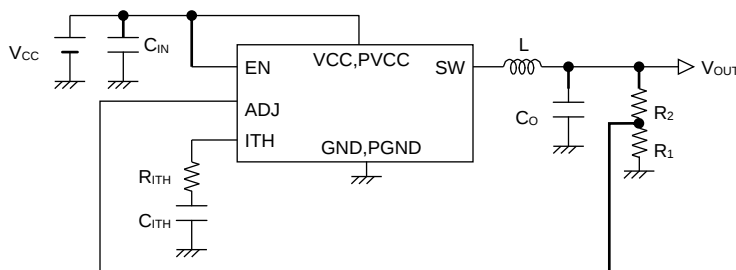
Figure 31. Typical Application Circuit
