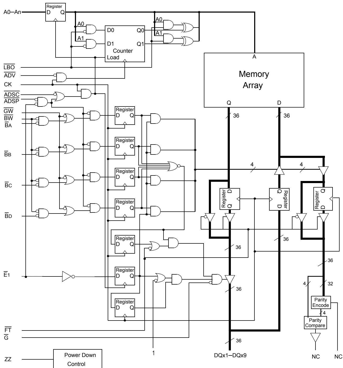
GS8321V18/32/36 Block Diagram
