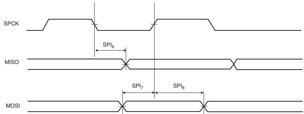
Figure 40-9. SPI Slave Mode with (CPOL=0 and NCPHA=1) or (CPOL=1 and NCPHA=0)
