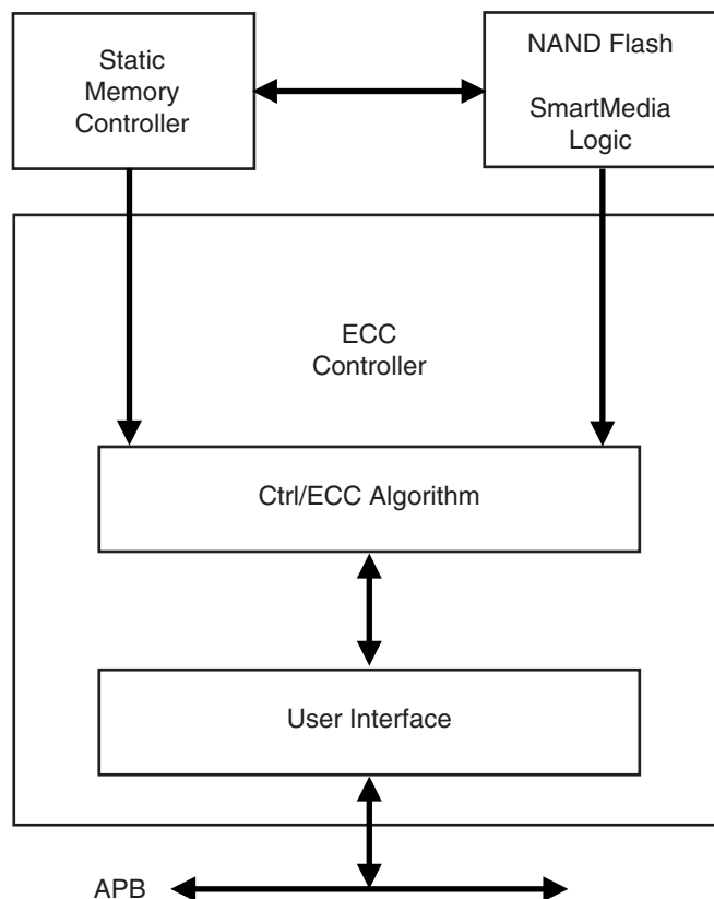
Figure 22-1. Block Diagram
