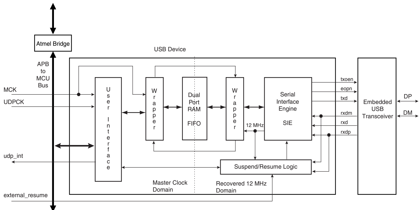
Figure 36-1. Block Diagram
