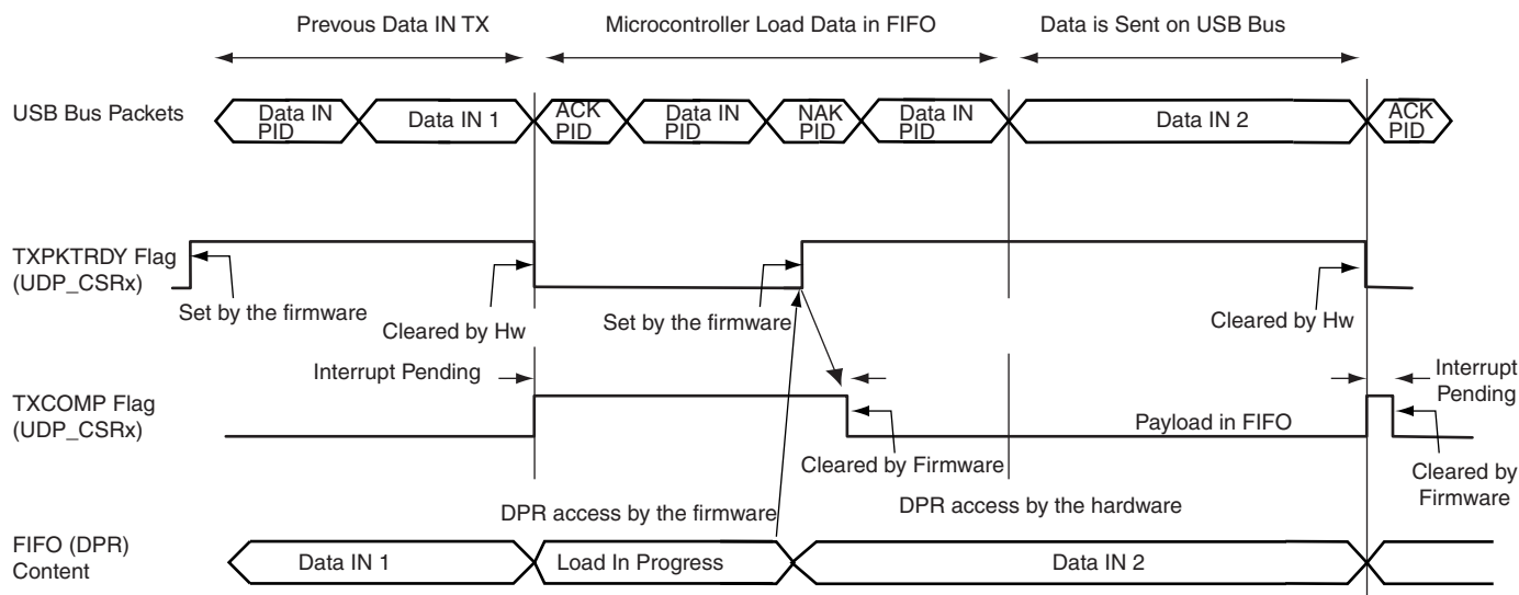
Figure 36-6. Data IN Transfer for Non Ping-pong Endpoint
