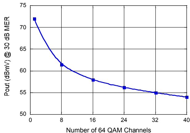
P_{OUT} @ 30 dB MER
