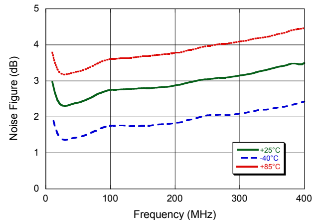
Noise Figure
