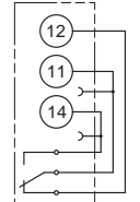
24 V DC Terminal Arrangement/ Internal Connections (Top View)
