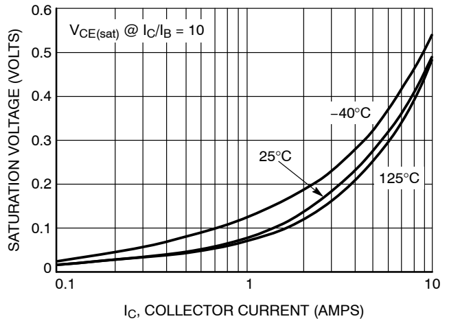
Figure 6. D45VH10 ON-Voltage
