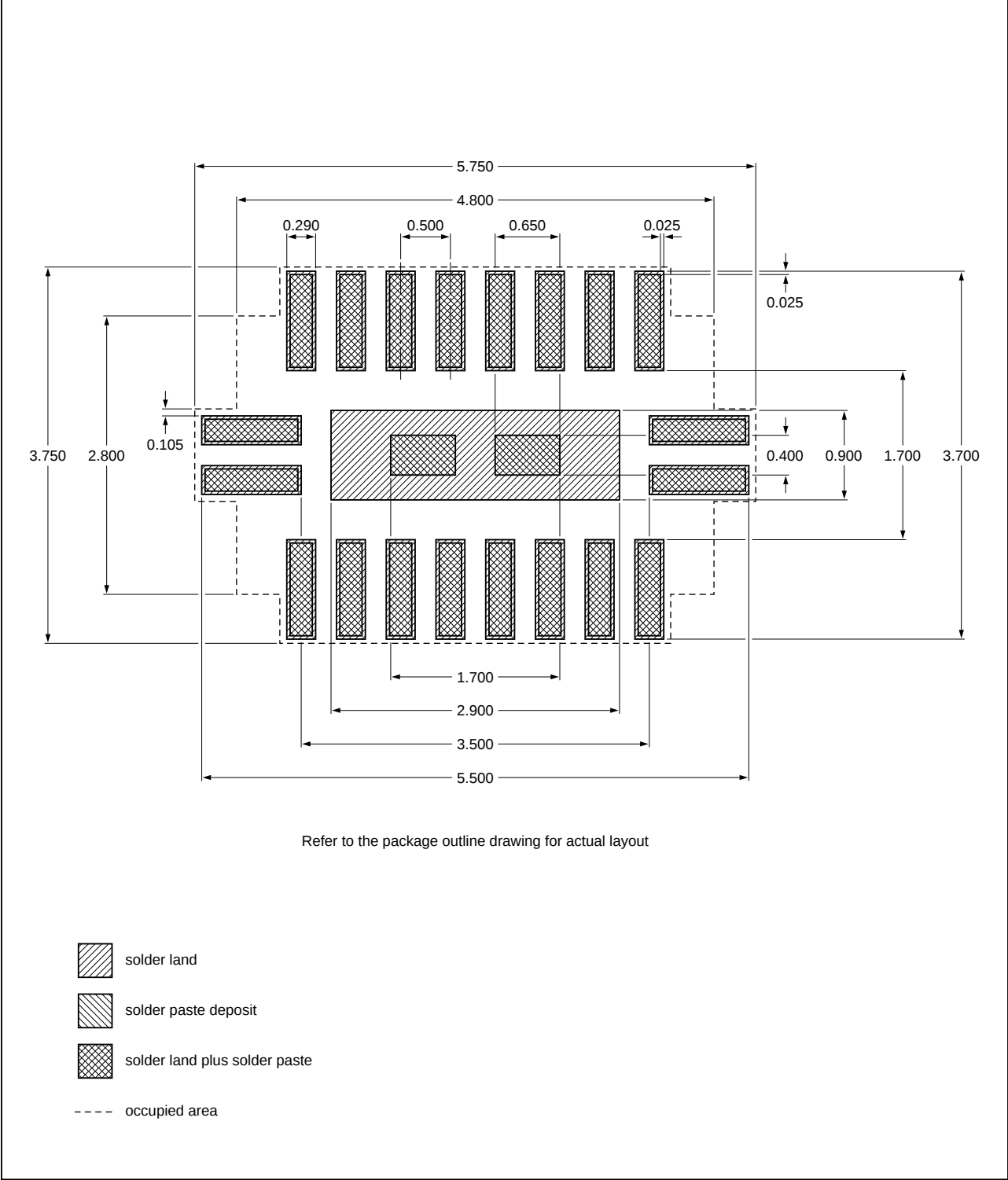
Fig 15. PCB footprint for SOT764-1 (TSSOP20); reflow soldering
