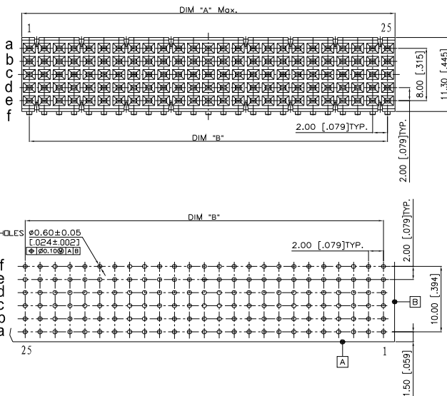
Reccommended PCB Layout
