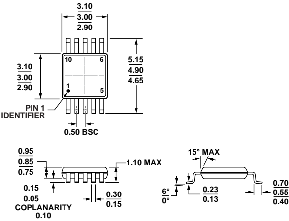
COMPLIANT TO JEDEC STANDARDS MO-187-BA Figure 46. 10-Lead Mini Small Outline Package [MSOP] (RM-10) Dimensions shown in millimeters
