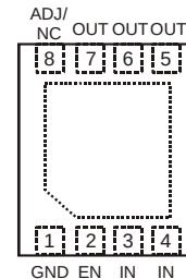
U-DFN2030-8
